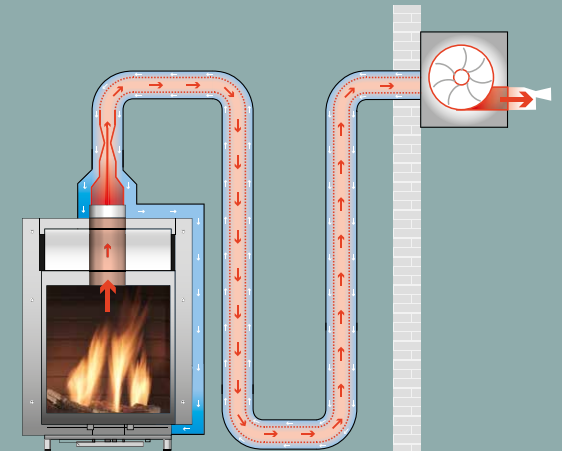
PowerVent®-System
